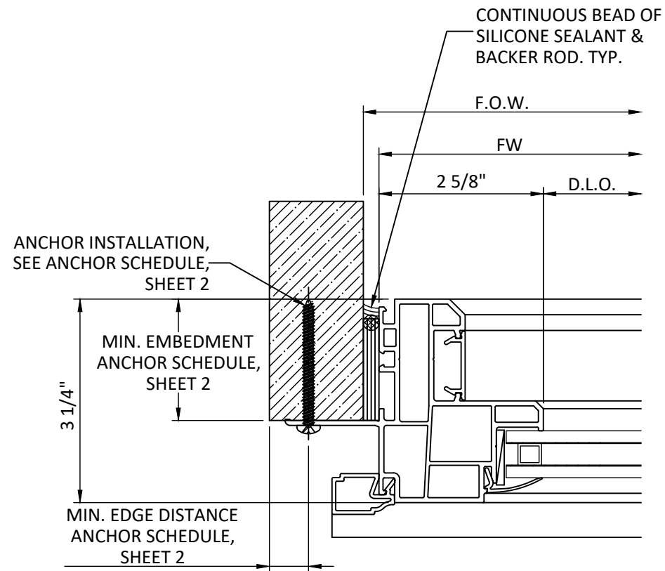
GLAZING DETAIL(1/1)
