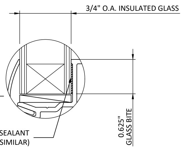
GLAZING DETAIL(1/1)
